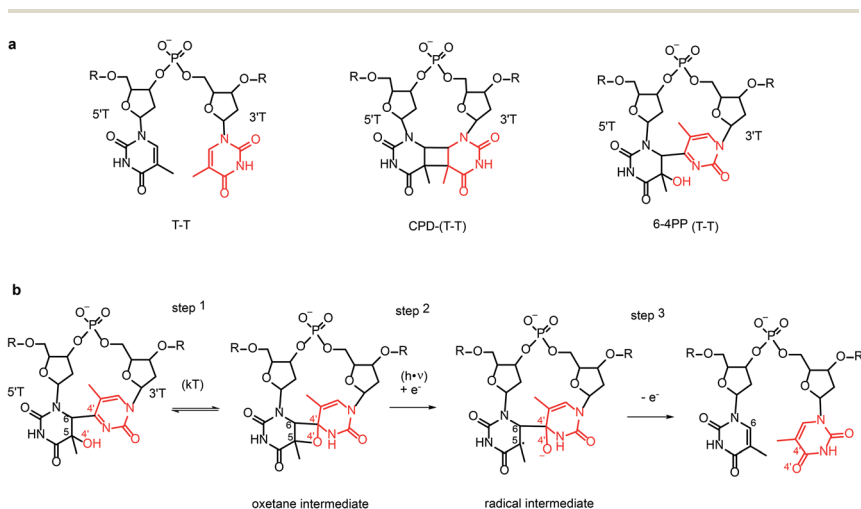
Scheme 1 (a) Chemical structure of the T–T dinucleotide and its CPD and 6–4 PP photolesions; (b) sequence of steps involved in the hypothesized repair of 6–4 PP photolesions by 6–4 photolyase via formation and photoreactivation of the oxetane intermediate. The atoms of the 3' base (3'T) are shown in red.
