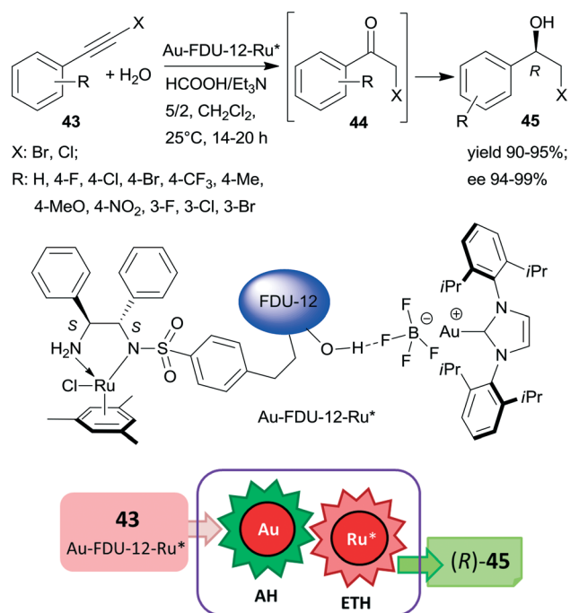
Scheme 13 Preparation of chiral haloalcohols 45 from haloalkynes 43 by tandem catalysis using large-pore mesoporous silica (FUD-12) immobilized Au-carbene and chiral Ru complexes. 129
