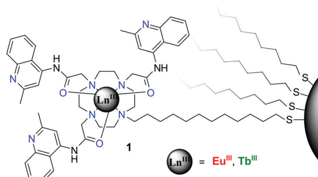
Fig. 25 The structure of AuNPs functionalised logic gate mimics, with two types of quinoline-cyclen complexes ( \text{Ln} = \text{Eu}^{\text{III}} or \text{Tb}^{\text{III}} ), functionalised to the Au-surface through thiol linkages.
