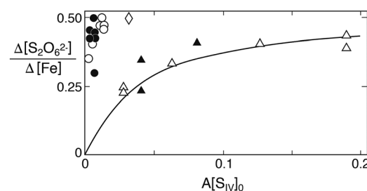
Fig. 9 Relative rate of dithionate production as a function of A[\text{S(IV)}_0] . Comparison of results obtained in different studies: circles A = 0.136 , points ( \text{Fe(II)} added) A = 0.078 (Pollard et al. 10 ); diamond, A = 6.22 (Dasgupta et al. 13 ); filled triangles, A = 2.04 (Higginson and Marshall 9 ); open triangles, A = 2.57 (Carlyle and Zeck 12 ). The solid line was calculated with k_4/k_3 = 45 .
