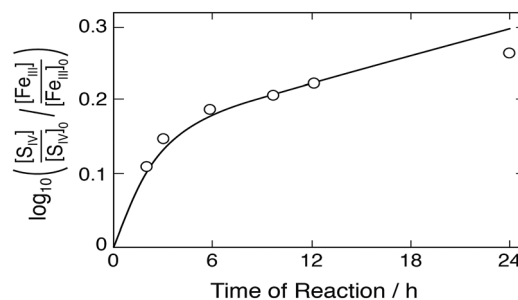
Fig. 8 Rate of the \text{Fe(III)}-\text{S(IV)} reaction (assumed to be bimolecular) as a function of time according to Pollard et al. 10 Points represent measurements, the solid line was calculated. Initial concentrations ( \text{mol dm}^{-3} ): [\text{Fe(III)}_0] = 0.2 , [\text{S(IV)}_0] = 0.0468 , [\text{H}^+] = 0.5 ; derived initial concentrations due to the presence of sulfates [\text{FeSO}_4^+] = 0.186 , [\text{Fe}^{3+}] = 0.0136 , [\text{HSO}_4^-] = 0.809 , [\text{SO}_4^{2-}] = 0.09 .
