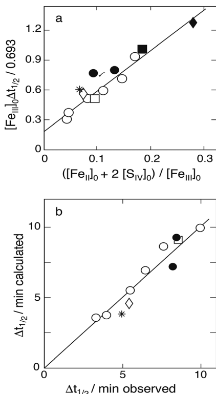
Fig. 7 (a) Plot of [\text{Fe(III)}_0\Delta t_{1/2}] versus ([\text{Fe(II)}_0 + 2[\text{S(IV)}_0]]/[\text{Fe(III)}_0]) to test the applicability of eqn (13b) in evaluating the data of Karraker; 11 initial concentrations ( \text{mmol dm}^{-3} ): [\text{S(IV)}_0] : 1.35–5.53, [\text{Fe(III)}_0] : circles 65.3, asterisk 89.0, open diamond 75.0, open square 13.1; [\text{Fe}^{2+}] added: points 0.9, solid square 4.93, solid diamond 11.4. The linear regression line excludes the marked point. (b) Comparison of calculated and measured reaction half-life times. The straight line is the 1:1 relation obtained with k_1/k_2 = 61.4 .
