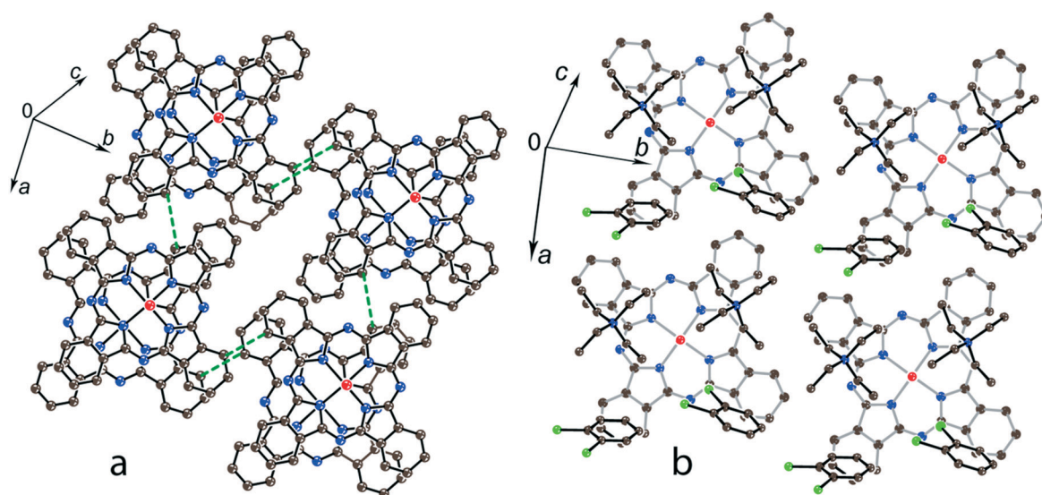
Fig. 2 (a) View of the phthalocyanine layer composed of the \pi -stacking [{Ti IV O(Pc 3- ) - }] 2 dimers in 1. 12 Short van der Waals C,N...C,N contacts are shown by green dashed lines. (b) Projection of the Et 4 N + ·C 6 H 4 Cl 2 layer on the phthalocyanine layer. Only one phthalocyanine from the dimer is shown (bonds are shown in grey).
