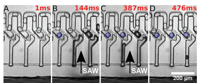
Fig. 2 SAW induced trapping of droplets. (A) No droplet enters the trap when no SAW is applied. (B) A SAW pulse at a specific position, controlled by the applied frequency, is injected. The SAW hits the coupling channel and a bubble is generated at this location. (C) When the SAW is shut off, the bubble collapses and droplets (marked blue) are loaded into the traps. Successive droplets are passing by the already loaded traps. A pulse length of 350 ms and a pulse power of 29 dBm were used.
