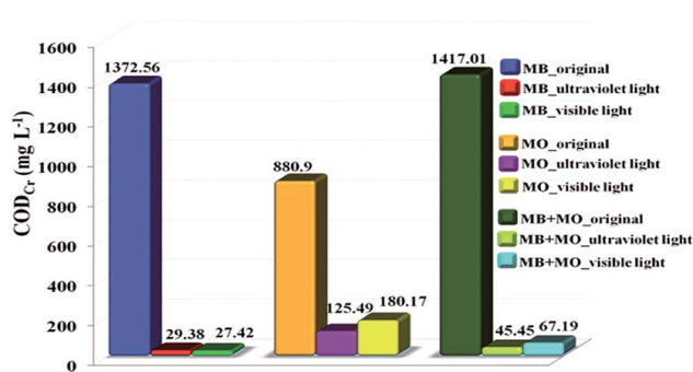
Fig. 11 The COD Cr changes of MB, MO and MB + MO mixture before and after UV or visible light irradiation in the presence of 1.
