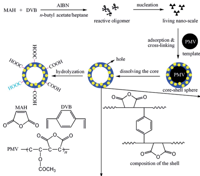
Fig. 9 Schematic of the strategy employed in the preparation of hollow spheres. Reproduced from ref. 94 with permission from the American Chemical Society.
