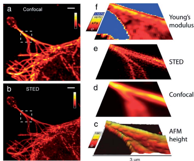
Fig. 6 Cos7 cells labeled with Atto 647 N, (a) confocal image, (b) STED image, (c) 3D AFM height image extracted from AFM force curves ( 45 \times 45 pixilated scan), (d) confocal image and (e) STED image (both linear deconvolved) (f) map of Young's modulus calculated from AFM force curves. Scale bars in (a) and (b): 2 μm, axes bars in (c)–(f): 3 μm. Reprinted from open-access article ref. 191 under the terms of the Creative Commons Attribution License.
