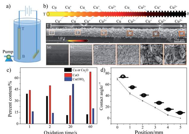
Fig. 1 Schematic of the formation of wettable gradient and Laplace pressure gradient on a copper wire and the change in the micro-structure, chemical composition, and water contact angle on Sample-A surface. (a) Apparatus for gradient anodic oxidation. (b) Schematic of the change in microstructure, chemical composition and SEM images of the copper wire surface (Sample-A). SEM images show that crisp and porous structures gradually appear after applying the gradient anodic oxidation process and the obvious directional roughness gradient is formed. In addition, the change in the diameter of the wire is also observed and a conical structure is formed (T: top area and B: bottom area of the copper wire during gradient anodic oxidation). (c) Chemical composition of copper wire prepared at different anodic oxidation time. The chemical composition gradient is also formed during the gradient anodic oxidation process. (d) Contact angles of Sample-A at different areas (the zero position is defined as the boundary between unoxidized part and oxidized part).
