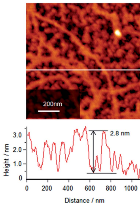
Fig. 4 AFM topographic image (tapping mode) of Cyt c /λ-DNA complex Langmuir monolayer transferred onto mica substrate at a surface pressure of 10 mN m -1 by horizontal dipping method. Barrier compression was done after 2 h of spreading Cyt c /λ-DNA mixed solution onto the subphase. Section profile of image shows the typical height of 2.8 nm which corresponds to the Cyt c /λ-DNA complex.
