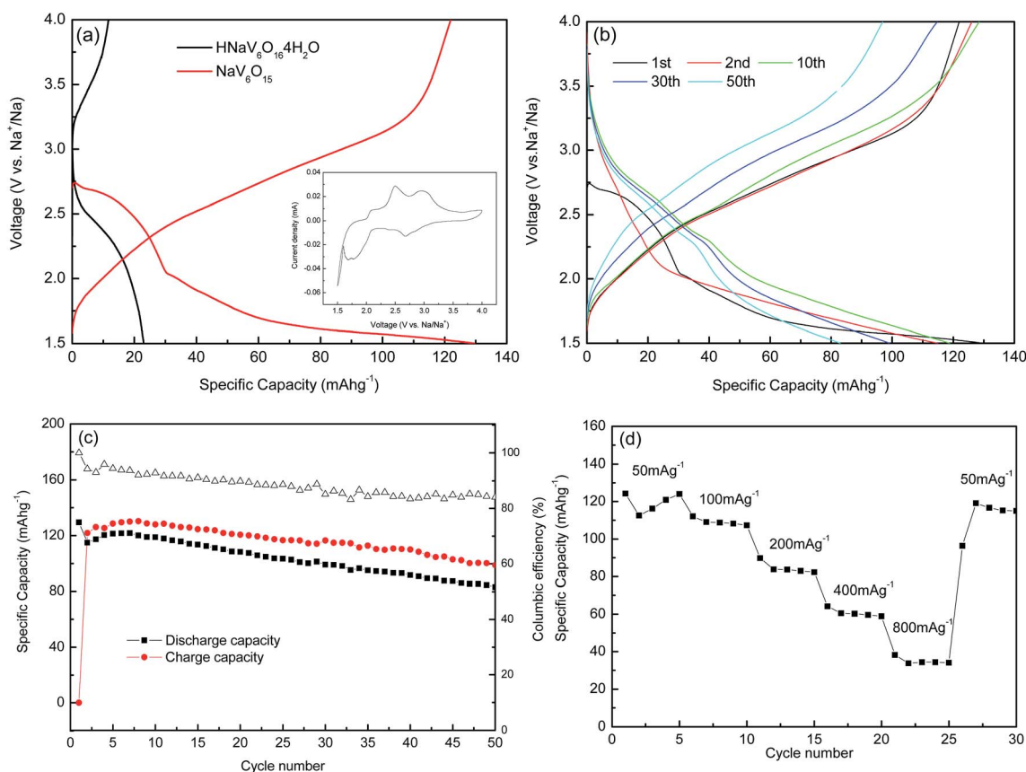
Fig. 7 (a) First charge–discharge profiles of \text{HNaV}_6\text{O}_{16} \cdot 4\text{H}_2\text{O} and \text{NaV}_6\text{O}_{15} microflowlers, the inset is CV curves of \text{NaV}_6\text{O}_{15}/\text{Na} (b) discharge/charge profiles of the selected cycles at the current density of 50 \text{ mA g}^{-1} (c) cycling performance of \text{NaV}_6\text{O}_{15} microflowlers at the current density of 50 \text{ mA g}^{-1} and the corresponding coulombic efficiency; (d) rate performance tested at different current densities.
