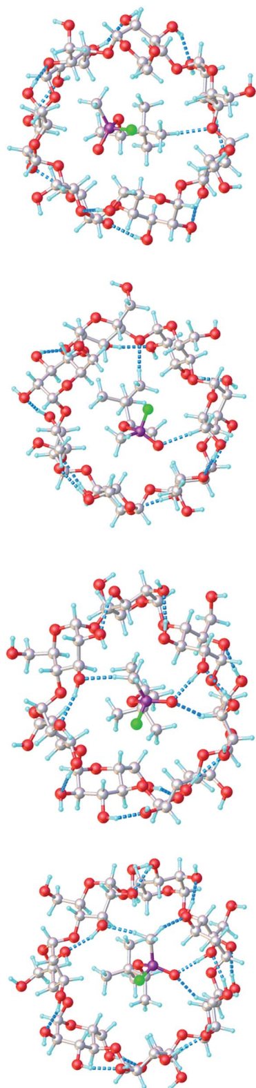
Fig. 8 \beta -CD \cdot GD complexes: (from top) C(-)P(+), C(+P)(+), C(+P)(-), C(-)P(-). Dashed lines indicate intermolecular interactions.
