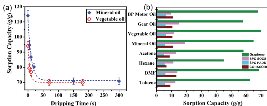
Fig. 3 Sorption capacity results of GA and the effect of drainage time. (a) GA sorption capacity decrease after the initial sorption of vegetable or mineral oil demonstrates that at least 1 minute of dripping or drainage after the oil sorption is required to represent the true sorption capacity of the graphene aerogel, (b) sorption capacities of the graphene aerogel for various oils and organic solvents and their comparison with commercial sorbents. The sorption capacities of the commercial sorbents Corksorb, Pads and SOCs are 6–14 \text{g g}^{-1} , 5–7 \text{g g}^{-1} and 10–20 \text{g g}^{-1} , respectively, which are much lower (more than 5 times) than that of the graphene aerogel with capacities of 40–70 \text{g g}^{-1} for various oils and organic solvents.
