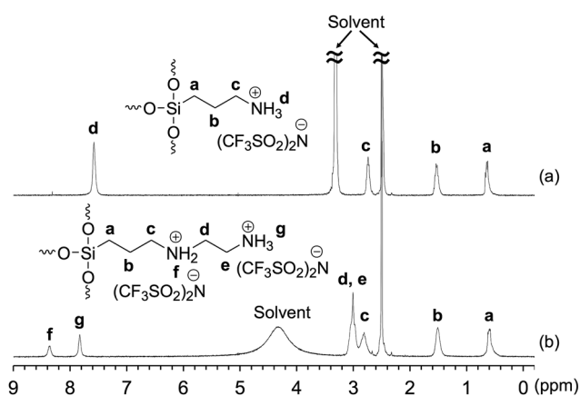
Fig. 10 1 H NMR spectra of (a) Am-POSS and (b) 2Am-POSS in DMSO- d 6 . Chemical shifts were referenced to DMSO (δ 2.5).
