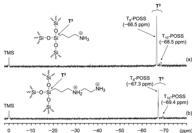
Fig. 12 29 Si NMR spectra of (a) Am-POSS and (b) 2Am-POSS in DMSO- d 6 at 40 °C. Chemical shifts were referenced to TMS (δ 0.0).
