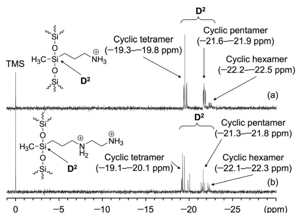
Fig. 4 ^{29}\text{Si} NMR spectra of (a) Am-CyS-IL and (b) 2Am-CyS-IL in DMSO- d_6 at 40 °C. Chemical shifts were referenced to tetramethylsilane (TMS; \delta 0.0).
