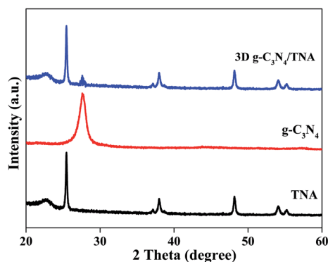
Fig. 4 XRD patterns for the 3D g-C 3 N 4 /TNA.
