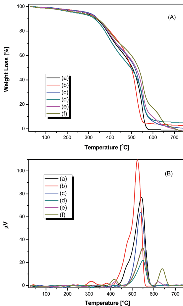
Fig. 5 TGA (A) and DTG (B) thermograms of pure polyazomrthine and its nanocomposites (a) pure PAMs, (b) PAMs/GNP a , (c) PAMs/GNP b , (d) PAMs/GNP c , (e) PAMs/GNP d and (f) PAMs/GNP f , in air at a heating rate of 10 °C min -1 .
