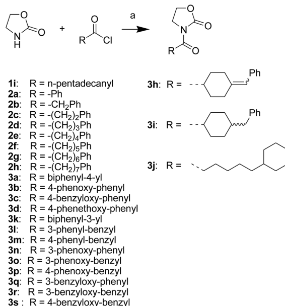
Scheme 6 The synthesis of compounds 1i , 2a–2h , 3a–3d and 3h–3s . Reagents and conditions: (a) n -BuLi, THF, -78\text{ }^\circ\text{C} .
