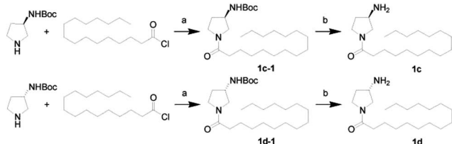
Scheme 4 The synthesis of compounds 1c and 1d . Reagents and conditions: (a) \text{Et}_3\text{N} , \text{CH}_2\text{Cl}_2 , room temperature; (b) \text{HCl} , dioxane, 0\text{ }^\circ\text{C} .
