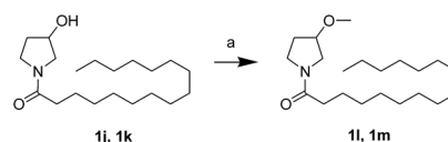
Scheme 2 The synthesis of compounds 1l and 1m . Reagents and conditions: (a) NaH , Mel , tetrahydrofuran (THF), 0^\circ C .
