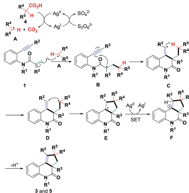
Scheme 5 Proposed mechanisms for forming products 3 and 5.
