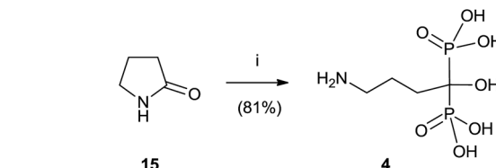
Scheme 3 Reagents and conditions: (i) H 3 PO 3 , PCl 3 . (ii) ArCOCl, NaOH.
