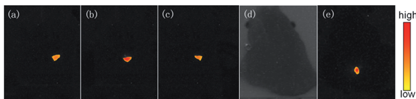
Fig. 9 NIR emission CCD pictures of the \text{Ba}_3(\text{VO}_4)_2:x \text{ mol}\% \text{Mn}^{5+} nanoparticles with doping concentration at (a) x = 0.5 , (b) x = 1 , (c) x = 1.5 . (d) Optical and (e) fluorescence images of \text{Ba}_3(\text{VO}_4)_2:1 \text{ mol}\% \text{Mn}^{5+} nanoparticles in pork tissue, excited by 808 nm laser.
