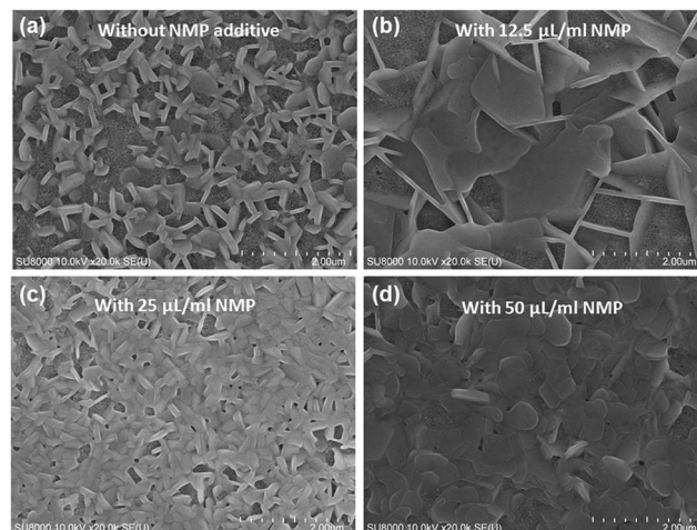
Fig. 1 Top surface SEM images of MBI perovskites without (a) and with different concentration of NMP additives (b–d).
