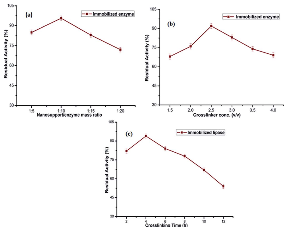
Fig. 1 Effects of immobilization parameters on activity of immobilized lipase. Effect of (a) nanosupport/enzyme mass ratio; (b) effect of crosslinker concentration; (c) effect of crosslinking time.
