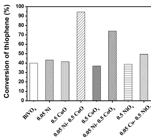
Fig. 6 Photocatalytic oxidation of thiophene on BiVO 4 and BiVO 4 loaded with various cocatalysts under visible light irradiation ( \lambda \geq 420 nm). Herein 0.5 Cu represents 0.5 wt% CuO/BiVO 4 , 0.05 Ni-0.5 Cu represents 0.05 wt% Ni-0.5 wt% CuO/BiVO 4 , and so on... Reaction conditions: [sulfur content] initial = 600 ppm; the concentration of photocatalyst: 1 g L -1 ; O 2 (bubbled into the system); temperature: 10 \pm 2 °C; reaction time: 3 h.
