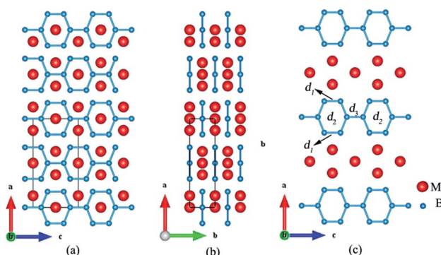
Fig. 3 Crystal structures of Immm\text{-MnB}_2 : (a) along the b -axis, (b) along the c -axis. (c) View of a one-layer structure of Immm\text{-MnB}_2 . The large red and small blue spheres represent Mn and B atoms, respectively.
