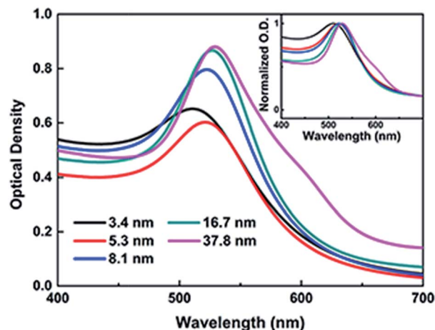
Fig. 4 UV-vis spectra of Au NPs with different diameters, and the normalized traces were in the inset.
