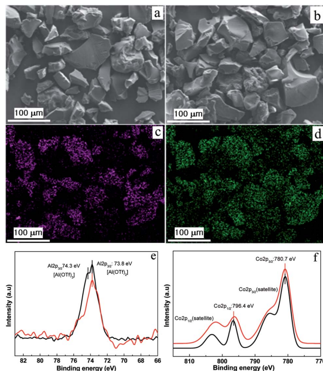
Fig. 2 SEM images of (a) 1 and (b) complex 3 . (c) Al and (d) Co elemental mappings of 3 . High-resolution XPS spectra of complex ( \rightarrow ) 4 and ( \leftarrow ) 3 (e) Al 2p peaks and (f) Co 2p peaks.
