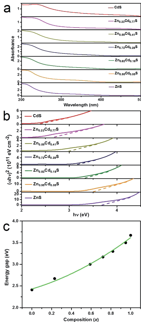
Fig. 4 (a) UV-visible optical absorption spectra of the \text{Zn}_x\text{Cd}_{1-x}\text{S} films with different composition x on a quartz substrate. (b) The variation of (\alpha h\nu)^2 as function of h\nu for the \text{Zn}_x\text{Cd}_{1-x}\text{S} films with different composition x . E_g can be attained by extrapolating the straight line plot of (\alpha h\nu)^2 versus (h\nu) to the energy axis. (c) E_g of the alloyed \text{Zn}_x\text{Cd}_{1-x}\text{S} films as a function of the composition x . It can be seen that the variation of E_g with composition x slightly deviates from linear dependence, displaying downward bowing.
