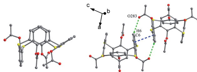
Fig. 96 Crystal structure of 109 (left), and a dimer of 109 (right) built by C–H···O and \pi – \pi interactions.
