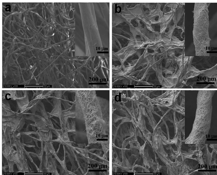
Fig. 2 SEM images of (a) cotton and cotton-AgNWs composites prepared by dipping cotton into an isopropanol solution of AgNWs (5.7 mg mL -1 ) for (b) one, (c) two, (d) three times, respectively.
