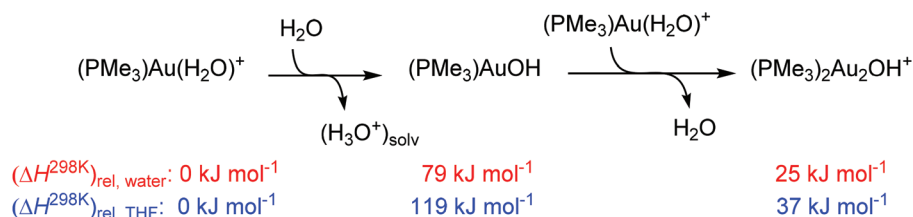
Scheme 2 Reaction of [(\text{PMe}_3)\text{Au}(\text{H}_2\text{O})]^+ with water.
