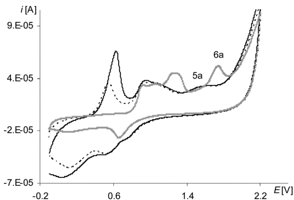
Fig. 8 Cyclic voltammograms of [Ni(salcn(Me)) in TBAH/CH 2 Cl 2 , 0–2.1 V, v = 0.05 \text{ V s}^{-1} , vs. Ag/AgCl; T = 293 \text{ K} ; gray line – 1st scan, dotted line – 2nd scan, solid black line – 3rd scan.
