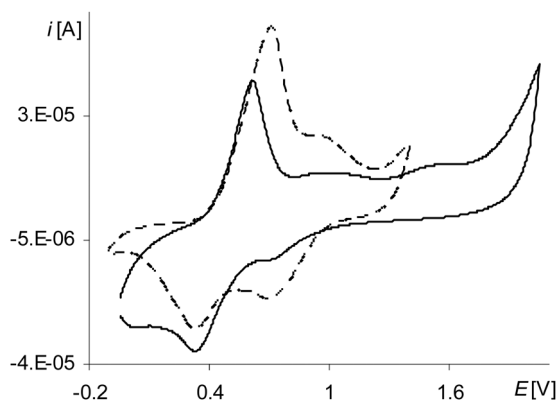
Fig. 7 Cyclic voltammograms of poly[Ni(salcn(Me)) in TBAH/CH 2 Cl 2 , 2nd scan, v = 0.05 \text{ V s}^{-1} , vs. Ag/AgCl; solid black line – after electropolymerization: 3 scans, 0–2.1 V, v = 0.05 \text{ V s}^{-1} ; dashed black line – after electropolymerization: 10 scans, 0–1.6 V, v = 0.05 \text{ V s}^{-1} .
