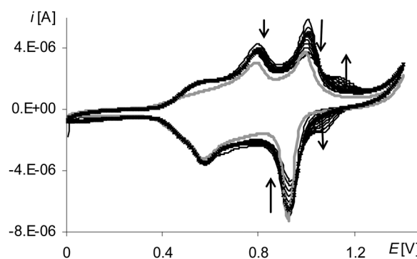
Fig. 10 Cyclic voltammograms of poly[Ni(salcn(Bu))] in TBAH/CH 2 Cl 2 , v = 0.05 \text{ V s}^{-1} , vs. Ag/AgCl; T = 293 \text{ K} ; black lines – 1st–10th scan after electropolymerization: 10 scans, 0–1.6 V, v = 0.05 \text{ V s}^{-1} ; gray line – 10th scan after electropolymerization: 3 scans, 0–2.1 V, v = 0.05 \text{ V s}^{-1} .
