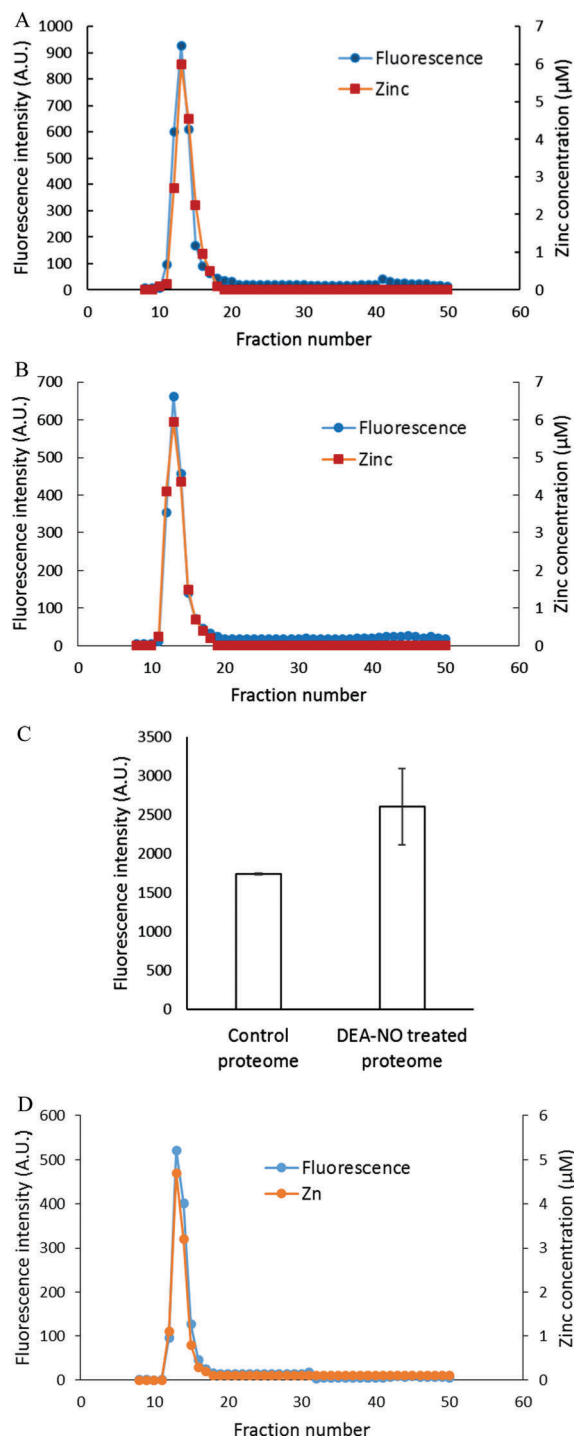
Fig. 6 Sephadex G-75 chromatography of LLC-PK 1 cell supernatant or isolated proteome incubated with TSQ followed by 500 \mu M DEA-NO. (A) 10^8 LLC-PK 1 cells were reacted with 500 \mu M DEA-NO for 45 min following 20 \mu M TSQ for 40 min. The cells were lysed, centrifuged, and the supernatant was separated using a Sephadex G-75 column. The fractions were analyzed for both fluorescence and zinc. (B) Control: a parallel reaction was run at identical condition with no DEA-NO added. (C) Comparison of the integrated fluorescence intensity of proteome. (D) Isolated proteome (10 \mu M Zn 2+ ) was reacted with 20 \mu M TSQ for 40 min followed by 500 \mu M DEA-NO for another 1 hour. The final reaction mixture was separated using a Sephadex G-75 column, and the fractions were analyzed for both fluorescence and zinc content. Error bars represent standard errors for at least three measurements.
