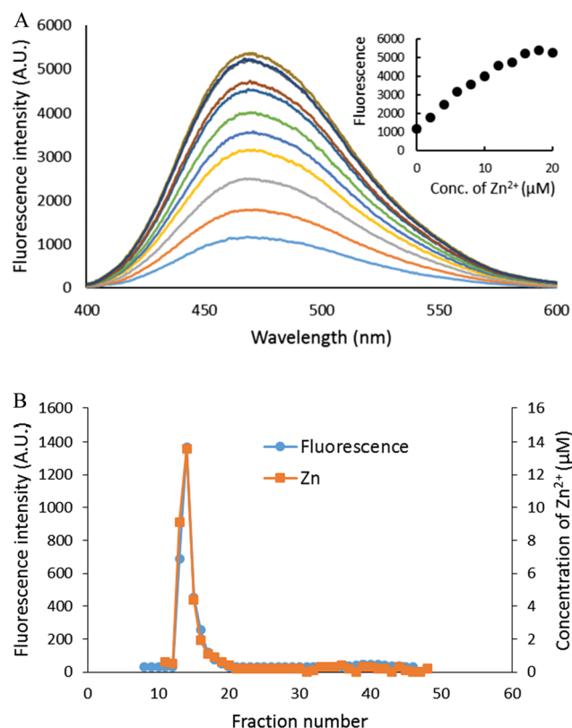
Fig. 7 Zn 2+ titration of proteome pre-treated with ZQacid. (A) Isolated proteome (8 \mu M Zn 2+ ) was reacted with 20 \mu M ZQacid for 30 min (the bottom most spectrum). Then, the reaction mixture was titrated with the increasing concentration of ZnCl 2 . (B) The final reaction mixture from (A) was fractionated using Sephadex G-75 gel filtration, and the eluted fractions were analyzed for both fluorescence and zinc content.
