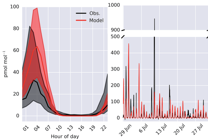
Fig. 6 Comparison of observed and modelled ("HAL") ClNO 2 as a median diel cycle (left) and timeseries (right) measured at Weybourne. Shaded regions on the diel plot give 25 th and 75 th percentiles.
