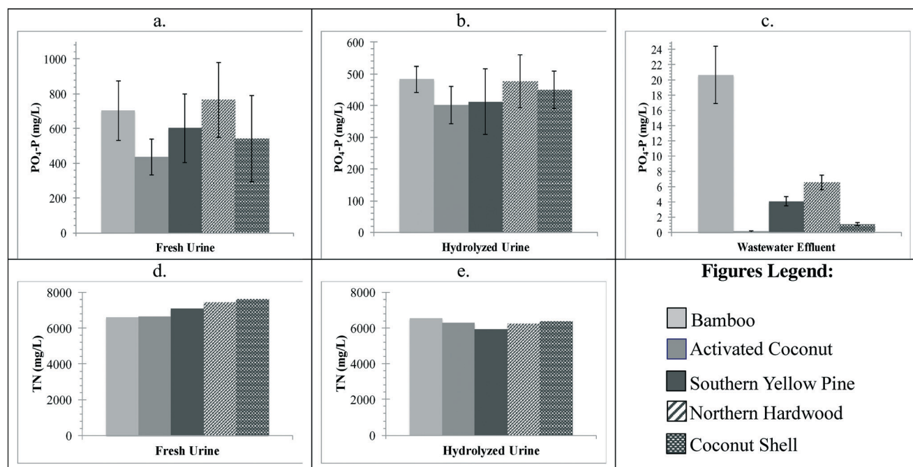
Fig. 3 Phosphate concentrations upon completion of batch tests at 40 g L -1 dose in a. fresh urine ( C_0 = 619 \text{ mg L}^{-1} \text{ PO}_4\text{-P} ), b. hydrolyzed urine ( C_0 = 438 \text{ mg L}^{-1} \text{ PO}_4\text{-P} ), and c. wastewater effluent ( C_0 = 1.54 \text{ mg L}^{-1} \text{ PO}_4\text{-P} ). Error bars indicate one standard deviation from seven sets of triplicate samples. Nitrogen removal by biochar for representative batches in d. fresh urine ( C_0 = 7362 \text{ mg L}^{-1} \text{ TN} ) and e. hydrolyzed urine ( C_0 = 7092 \text{ mg L}^{-1} \text{ TN} ).
