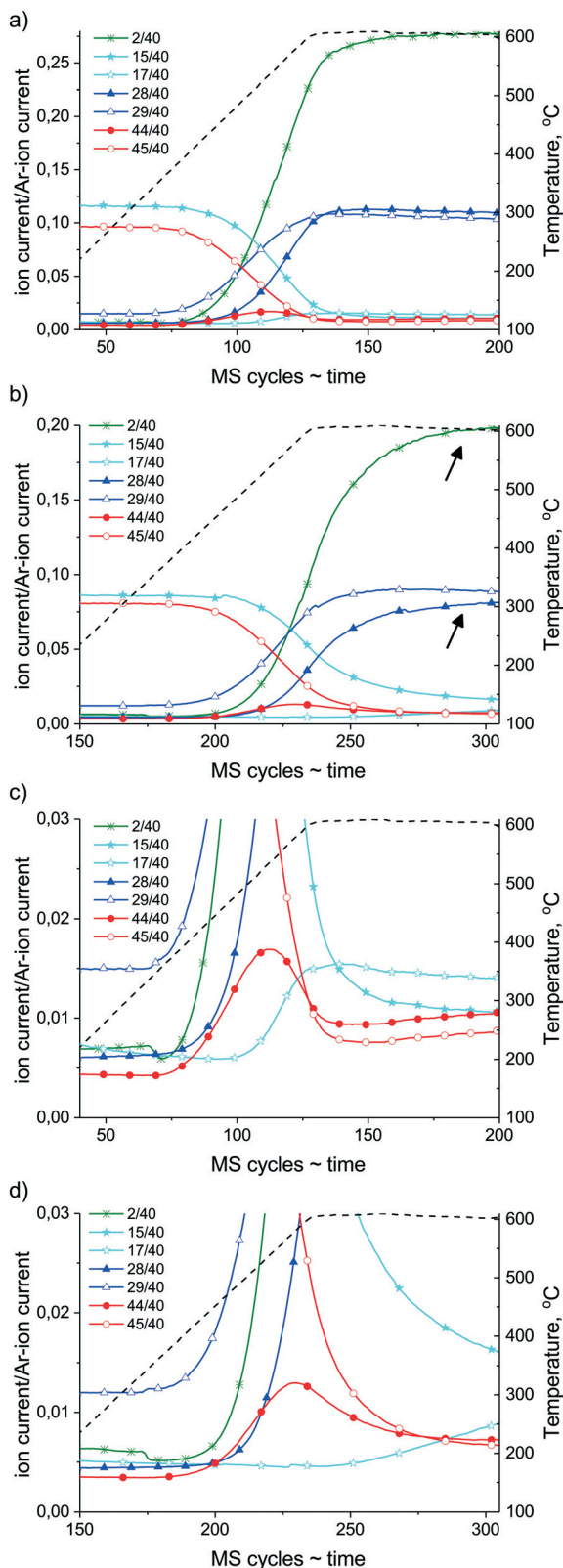
Fig. 9 Ramp-hold type dry reforming reaction with a ^{13}\text{CO}_2 : ^{12}\text{CH}_4 = 1 mixture in the closed loop circulation system on (a) \text{Ni}/\text{ZrO}_2 and (b) \text{Na-Ni}/\text{ZrO}_2 . (c) Enlargement of low intensity signals of spectrum “a” and (d) enlargement of low intensity signals of spectrum “b”. Conditions: \sim 25 mbar each reactant ( ^{12}\text{CH}_4 contains 2% Ar), temperature ramp with 10^\circ\text{C min}^{-1} up to 600^\circ\text{C} then isothermal 30 min at 600^\circ\text{C} . 1 MS cycle = 26 s.
