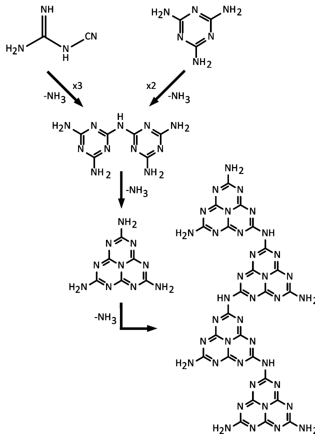
Fig. 5 Sequence of polymerization reactions proposed for dicyandiamide or melamine leading to Liebigs melon via condensation and elimination of NH_3 components. Further condensation reactions could ultimately lead to sideways cross-linking of polyheptazine ribbons to form sheet-like structures, but no fully polyheptazine based g- C_3N_4 has been observed to date.
