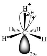
Scheme 3 A schematic representation of \text{C}_2\text{H}_5^+ \cdots \text{Ar} ( C_{3v} , Ar is omitted) along the C–C bond. Dihedral angle \theta shows deviation of the \text{C-C-H}^+ plane from the direction of carbon's 2p_z orbital.
