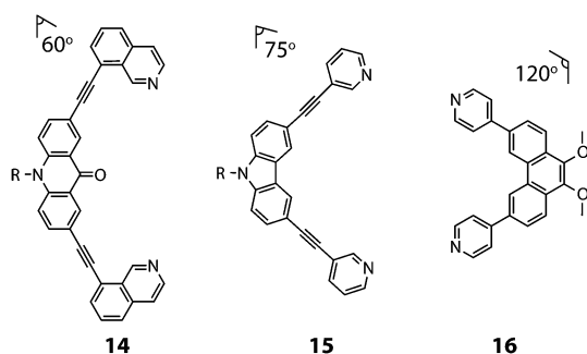
Fig. 9 The angularly distinct bis-monodentate ligands ( 14–16 ) used to assemble [\text{Pd}_2\text{L}_2\text{L}_2]^{4+} heteroleptic cages ( \text{R} = \text{C}_6\text{H}_{13} ).
