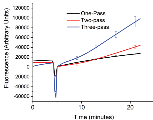
Fig. 3 Signal enhancement from multiple-pass target recycling. A 5\ nM target DNA was added to a solution containing 50\ nM of either only P_0A_1A_2 (one-pass), both P_0A_1A_2 and P_1S (two-pass), or P_0A_1A_2 , P_1S , and P_2S (three-pass) and the reaction buffer mixture ( 1\times NEBuffer 1 with 50\ mM\ Mg^{2+} ) and 20\ \mu L\ 1\ U\ \mu L^{-1} of exo\ III . The fluorescence signal was measured every 15 seconds at room temperature. (At t = \sim 5 , the signal dropped because the spectrofluorometer was opened when exo\ III was added.)
