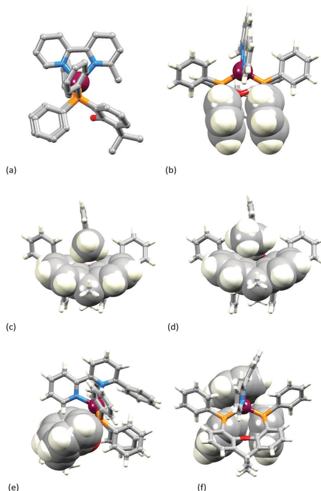
Fig. 3 (a–c) The structure of the [Cu(xantphos)(Mebpy)] + cation: (a) view along the P–P vector of the xantphos ligand (H atoms omitted for clarity); (b) face-to-face \pi -stacking of phenyl rings in the two different PPh 2 units; (c) accommodation of the methyl group of Mebpy in the xantphos 'bowl'. (d) A view of the [Cu(xantphos)(Etbpy)] + cation for comparison with the analogous view of [Cu(xantphos)(Mebpy)] + shown in (c). (e and f) The structure of the [Cu(xantphos)(Phbpy)] + cation with space-filling representations emphasizing (e) the xanthene 'bowl' with the unsubstituted pyridine ring lying above it, and (f) the phenyl group of Phbpy oriented over two Ph rings of the PPh 2 units.
