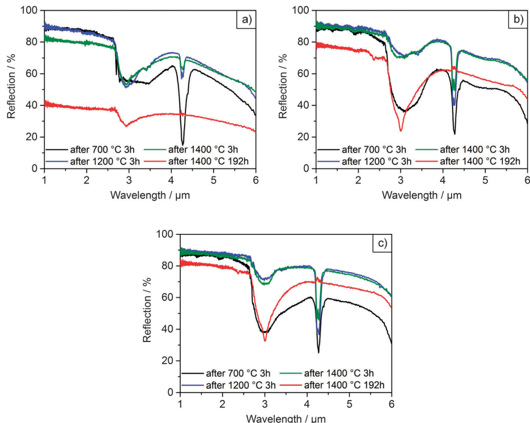
Fig. 6 Diffuse reflectance spectra of films F0 (a), F6 (b) and F10 (c) after selected heating cycles.
