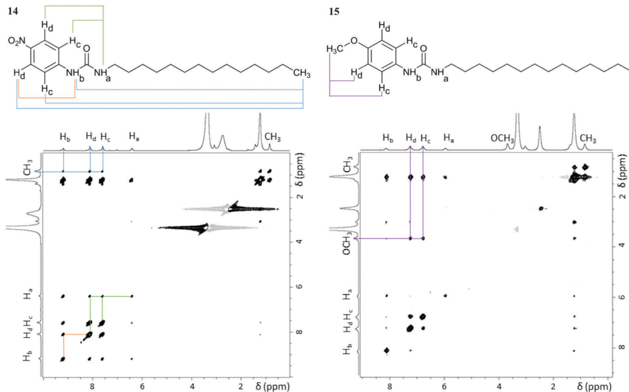
Fig. 6 2D ^1\text{H} - ^1\text{H} NOESY spectra of gels 14 and 15 ( 60\text{ mg mL}^{-1} in \text{DMSO}-d_6 ) acquired at 25^\circ\text{C} with a mixing time of 0.5\text{ s} using a 800.23\text{ MHz} spectrometer. Relevant cross-peaks have the corresponding spatial connectivity assigned (coloured lines). The cross-peaks observed between the -\text{CH}_2 and the aromatic protons in gel 15 do not contain structural information, as they result from indirect NOE enhancements, only observable at long mixing times (ESI†).
