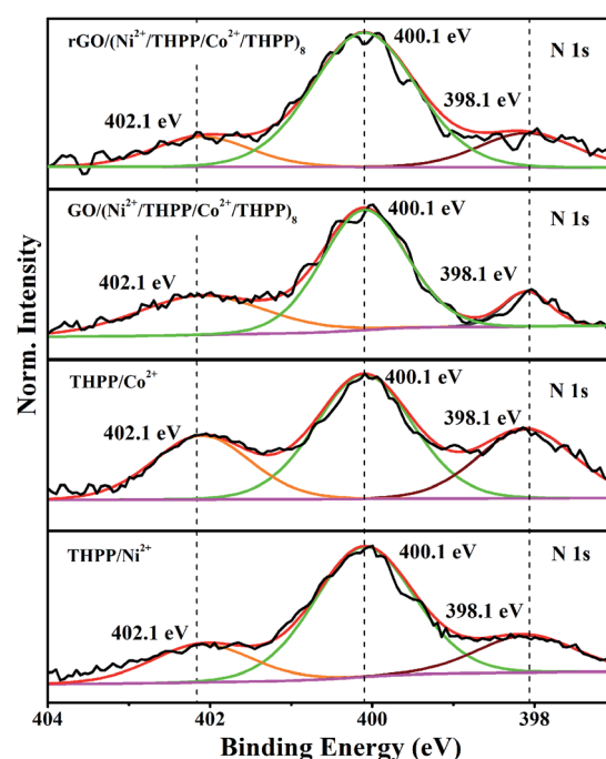
Fig. 2 High-resolution XPS spectra of N 1s of \text{THPP}/\text{Ni}^{2+} , \text{THPP}/\text{Co}^{2+} , \text{GO}/(\text{Ni}^{2+}/\text{THPP}/\text{Co}^{2+}/\text{THPP})_8 and \text{rGO}/(\text{Ni}^{2+}/\text{THPP}/\text{Co}^{2+}/\text{THPP})_8 .
