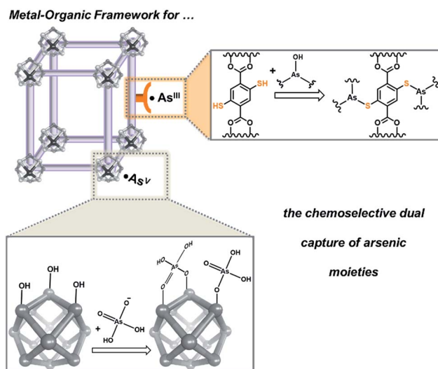
Fig. 1 A schematic representation that suggests how MOFs can be tailored to coordinate anionic \text{As}^{\text{V}} moieties at the node while binding neutral \text{As}^{\text{III}} with the linkers.
