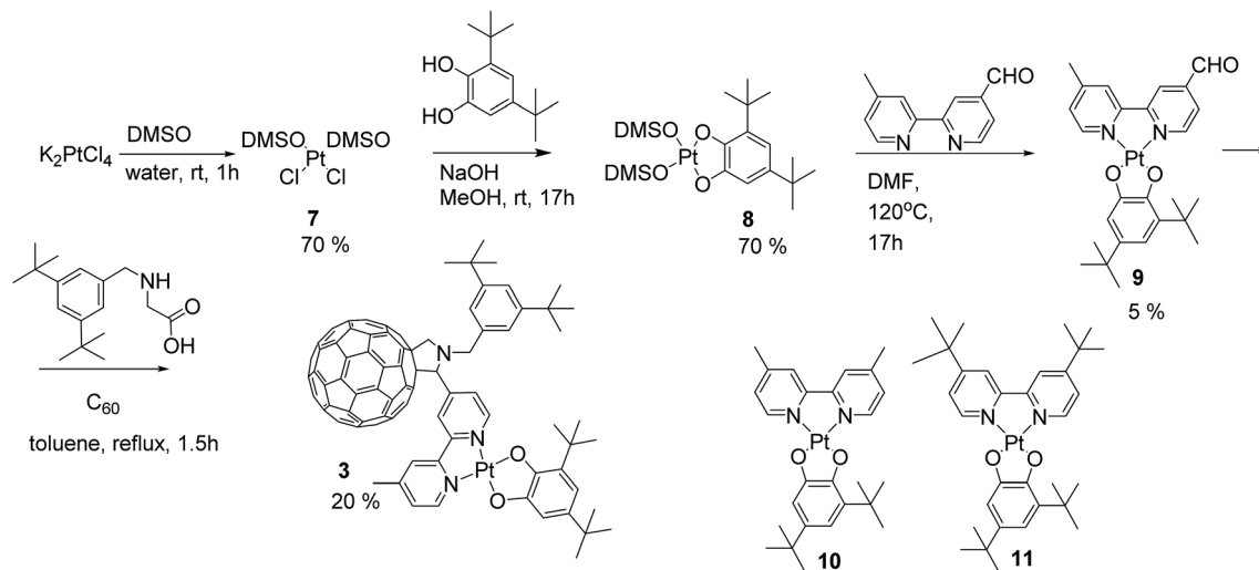
Scheme 2 Alternative synthetic route towards the donor-acceptor complex 3 via the Prato reaction of the aldehyde group tagged bipyridine-Pt-catechol unit and \text{C}_{60} fullerene. Molecular structures of the model dyads (4,4'-diMe-bpy)Pt(cat) ( 10 ) and (4,4'-di t Bu-bpy)Pt(cat) ( 11 ) are also shown.
