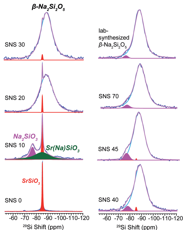
Fig. 1 29 Si MAS NMR spectra of Na-doped SrSiO 3 (with apparent composition of Na x Sr 1-x SiO 3-0.5x ) with different Na contents ( x = 0, 0.1, 0.2, 0.3, 0.4, 0.45 and 0.70, denoted as SNS0, SNS10, SNS20, SNS30, SNS40, SNS45 and SNS70, respectively) and lab-synthesized β-Na 2 Si 2 O 5 . Relevant resonance assignments, including SrSiO 3 (red), SrSiO 3 with Na doped within the structure (Sr(Na)SiO 3 , green), Na 2 SiO 3 (magenta), and β-Na 2 Si 2 O 5 (blue) are marked on the spectra. Spectral simulations are displayed together with the experimental spectra. All the NMR parameters used for the simulations are listed in Table S1.†
