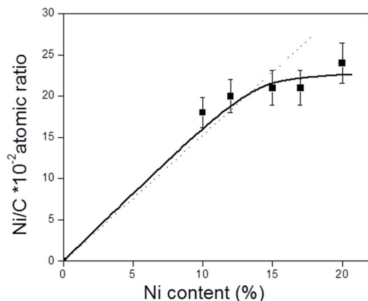
Fig. 3 Relationship between Ni/C atomic ratio obtained from XPS analysis and Ni content (% wt) of the x\text{Ni}/\text{CNT} catalysts. The dotted line represents the theoretical values.
