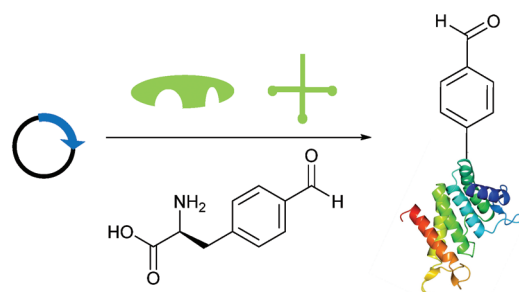
Scheme 8 Installation of aldehyde into proteins via unnatural amino acid mutagenesis. Expression of a plasmid encoding for the desired protein containing an amber STOP codon in conjunction with an orthogonal tRNA synthetase/tRNA pair and unnatural amino acid allows for incorporation of an aldehyde-containing amino acid at the aforementioned STOP position.
