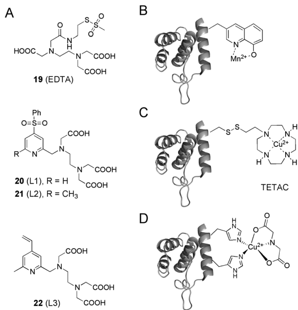
Fig. 5 Labels and labeling strategies to introduce \text{Mn}^{2+} or \text{Cu}^{2+} cations into proteins.
